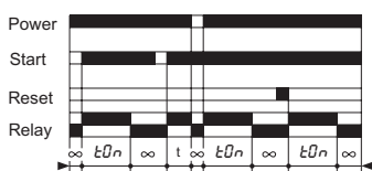
Config. 7 Timing on energization
