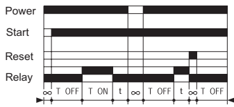
Config. 5 Cyclic timing
