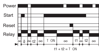
Config. 3 Timing on impulse (one shot)
