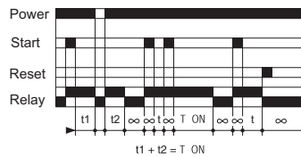
Config. 4 Timing after impulse (delay off)
