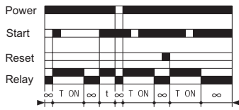
Config. 3 Timing on impulse (one shot)
