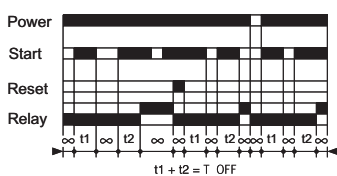
Config. 8 Timing on energization with memory
